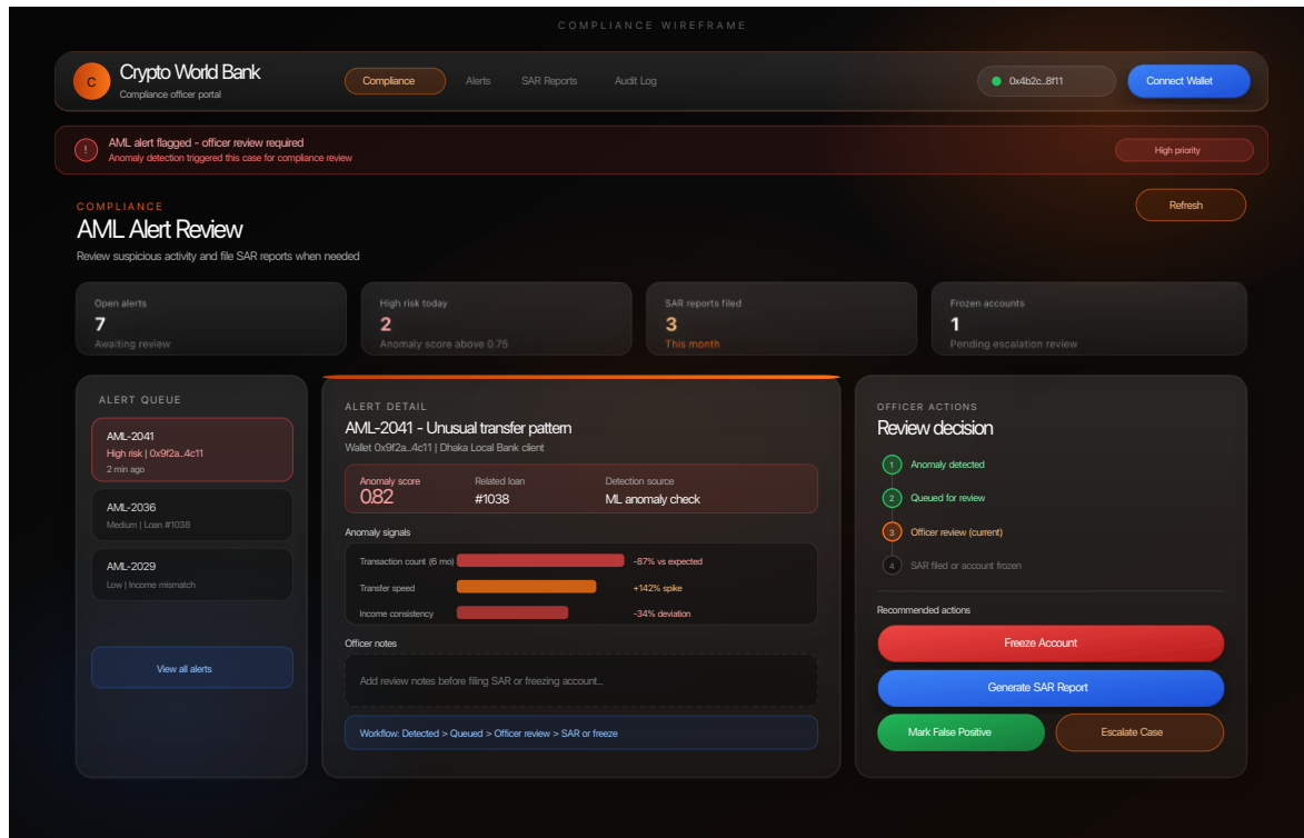
Figure 4.39: Compliance wireframe.
