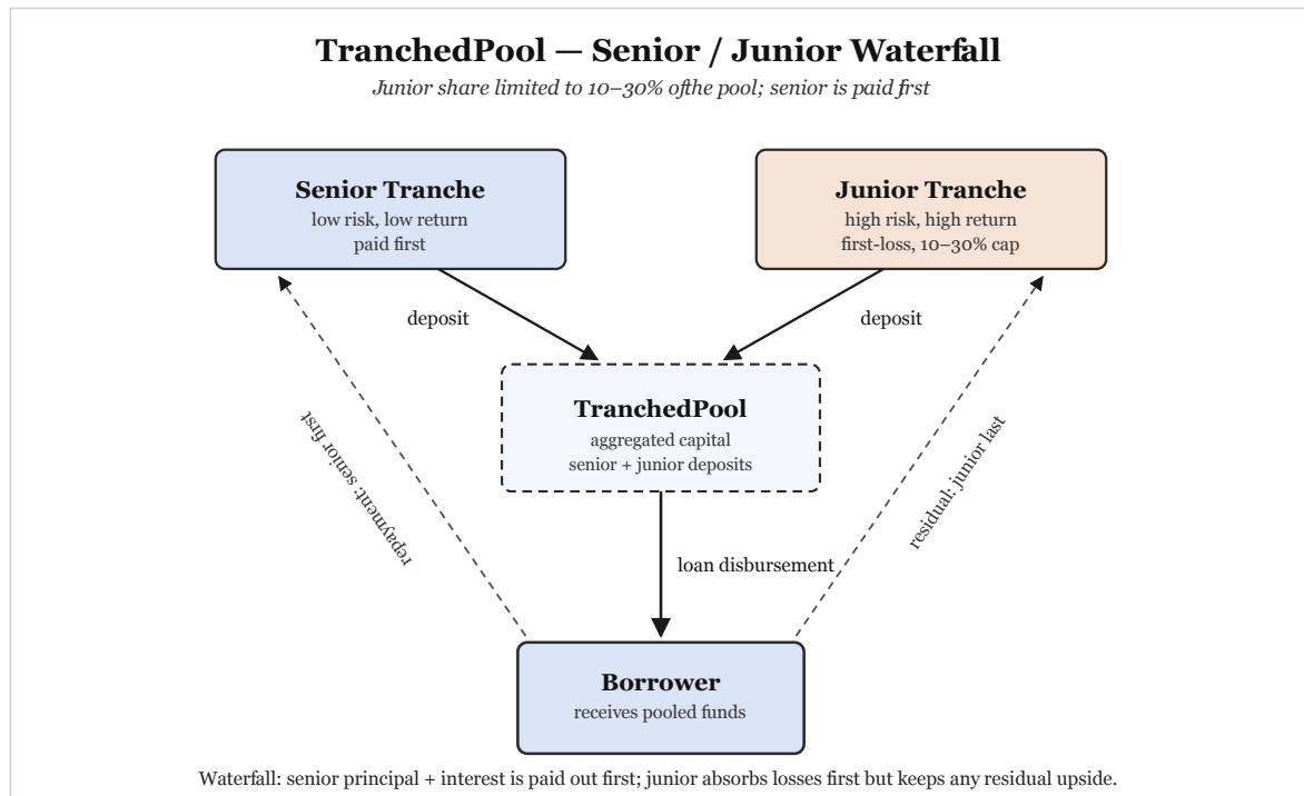
Figure 4.19: TranchedPool.
