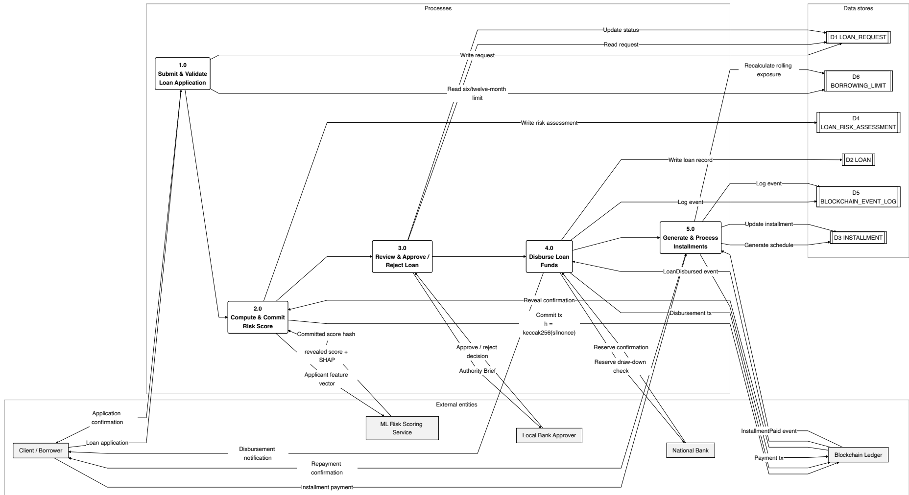
Figure 4.27: DFD Level 1.
