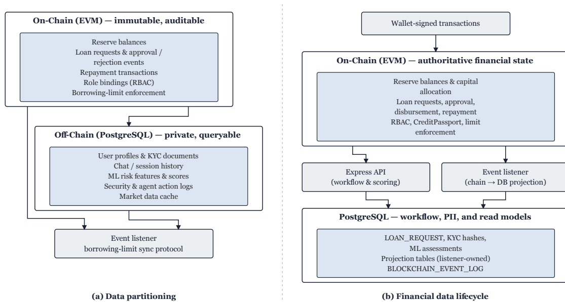
Figure 4.10: Data partitioning and financial data lifecycle.
