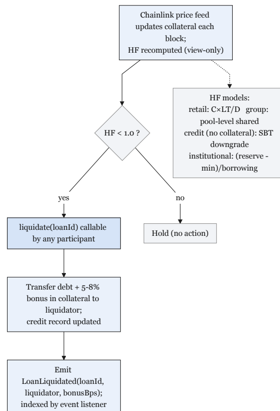
Figure 4.13: Liquidation engine.
