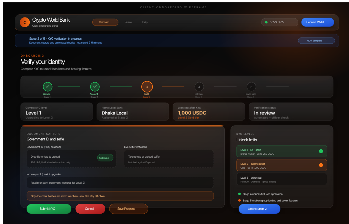
Figure 4.35: Onboarding wireframe.
