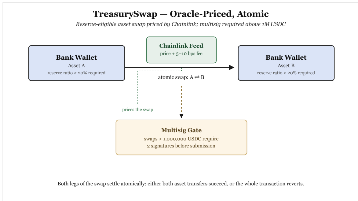
Figure 4.20: TreasurySwap.
