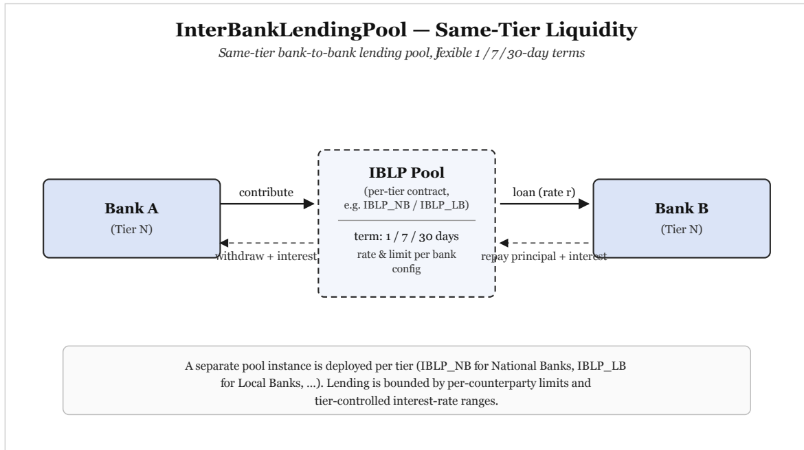
Figure 4.16: InterBankLendingPool.
