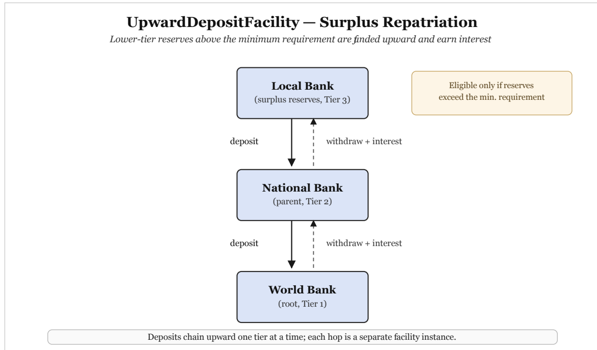
Figure 4.17: UpwardDepositFacility.
