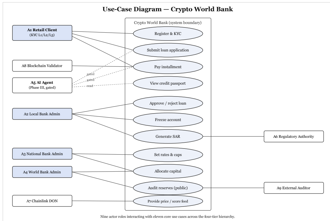
Figure 4.22: Use-case diagram.
