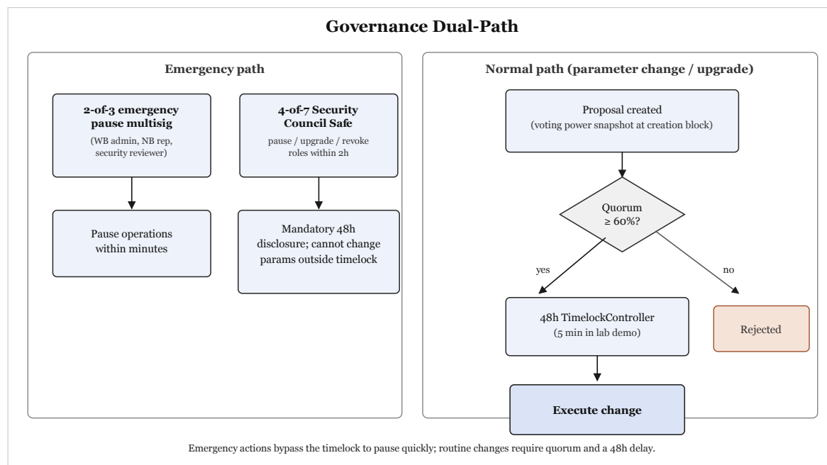
Figure 4.42: Governance dual-path.
