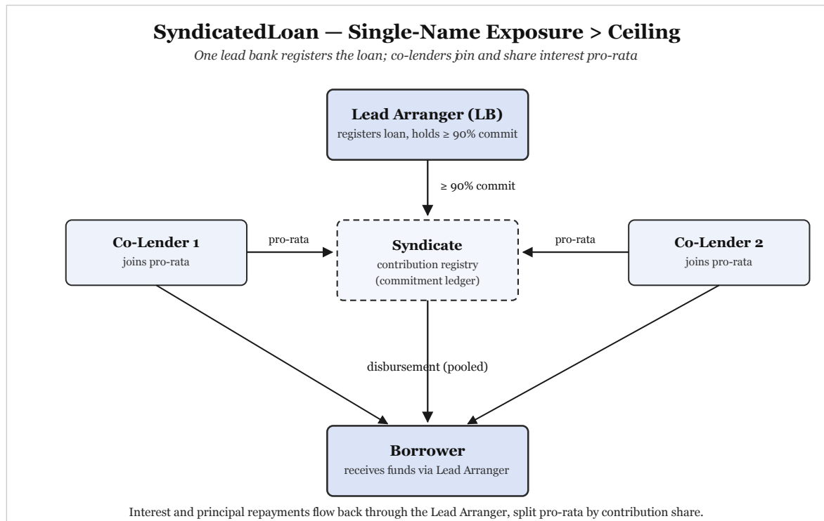
Figure 4.18: SyndicatedLoan.
