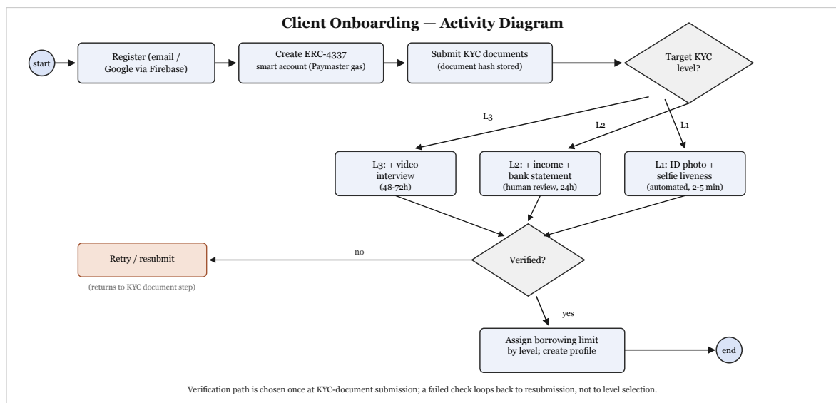
Figure 4.24: Onboarding activity.
