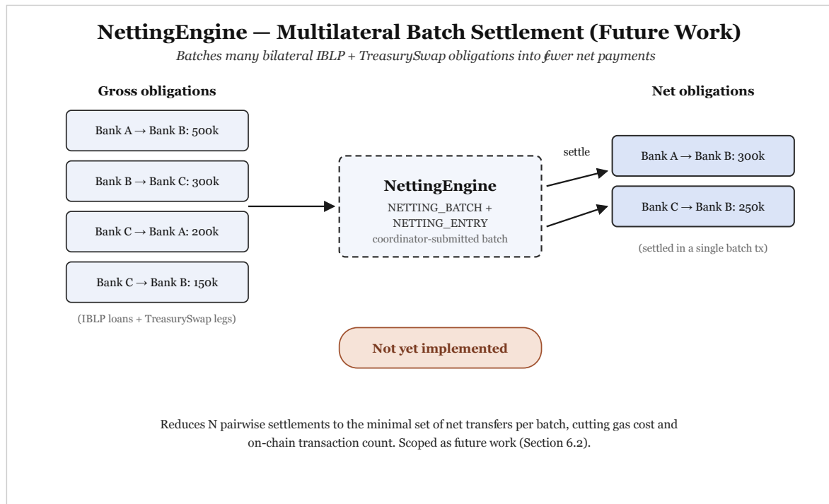
Figure 4.21: NettingEngine.
