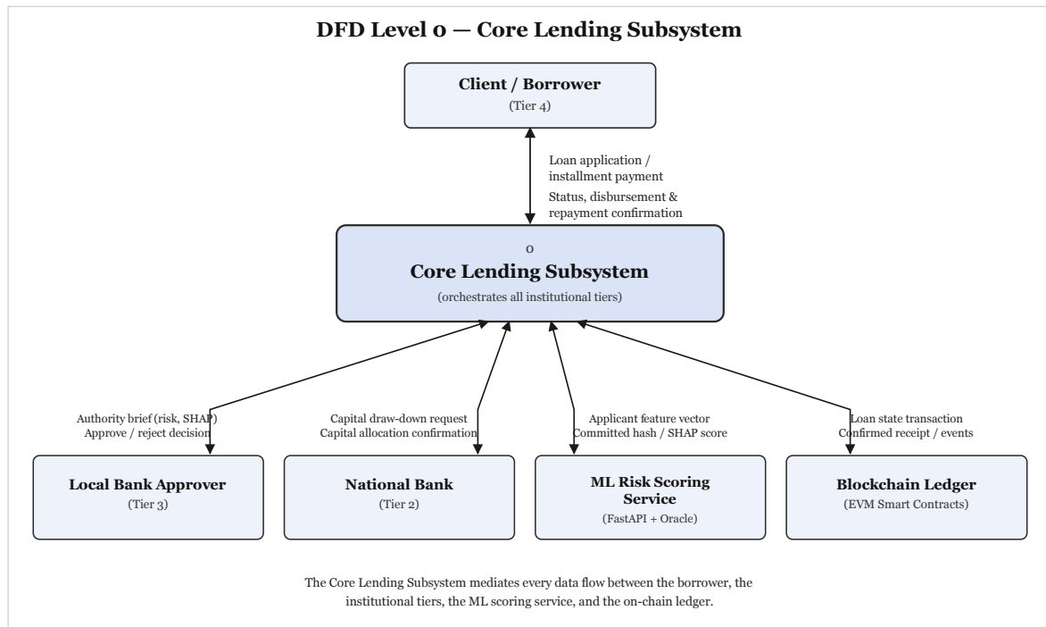
Figure 4.26: DFD Level 0.
